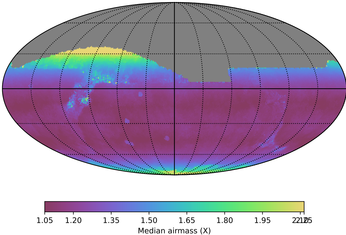
mw_roll_all_v3.3_10yrs All sky z band: Median airmass
