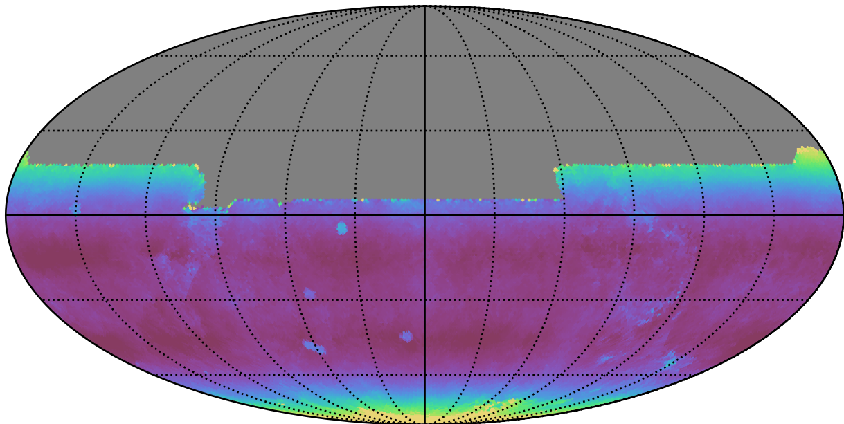
mw_roll_all_v3.3_10yrs All sky y band: Median airmass
