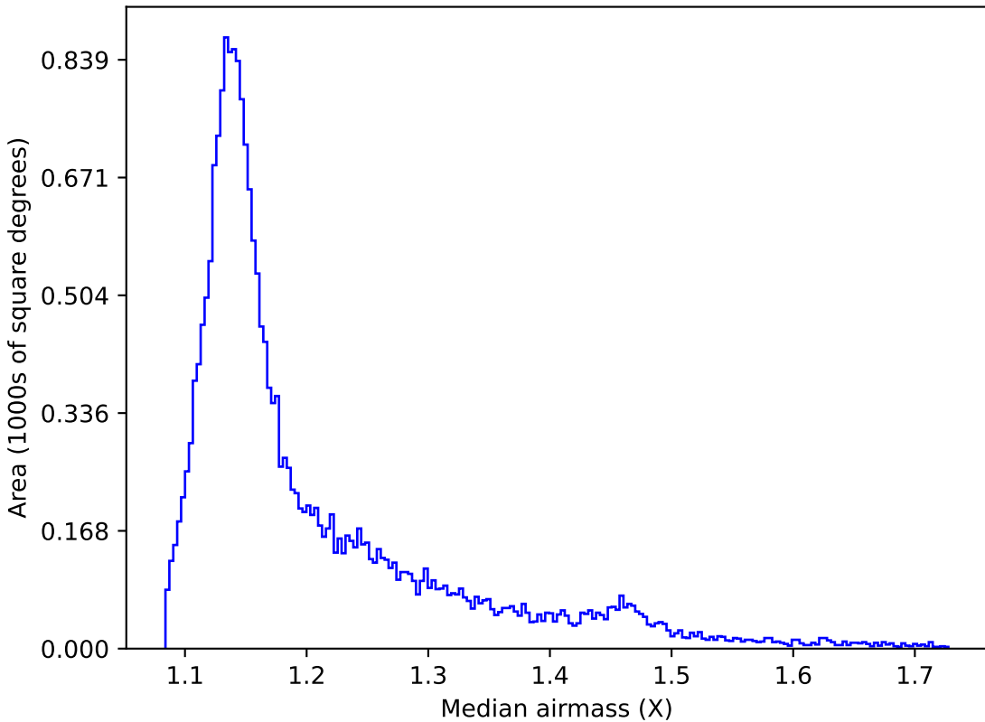
mw_roll_all_v3.3_10yrs All sky y band: Median airmass
