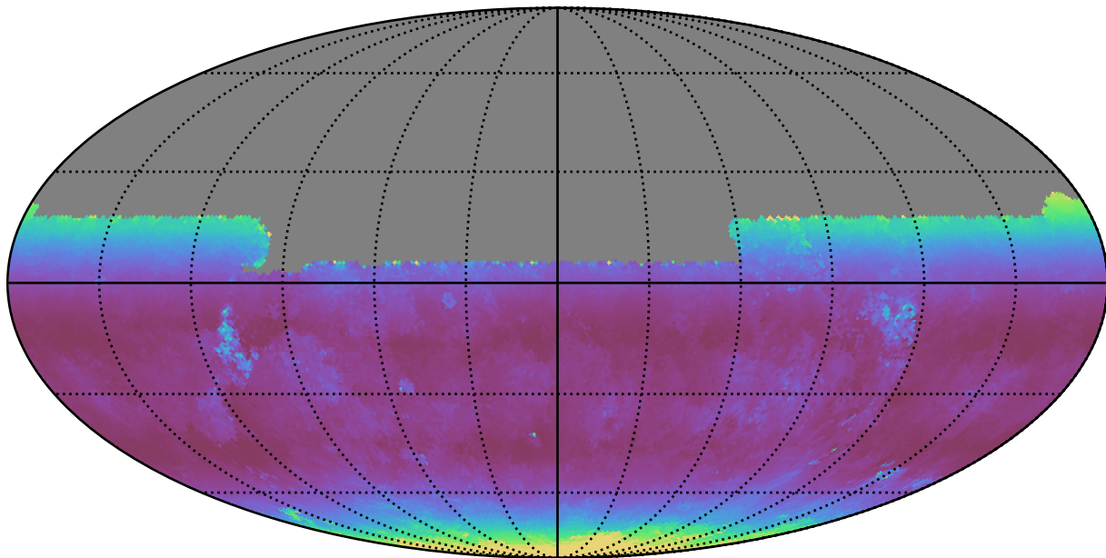
mw_roll_all_v3.3_10yrs All sky u band: Median airmass
