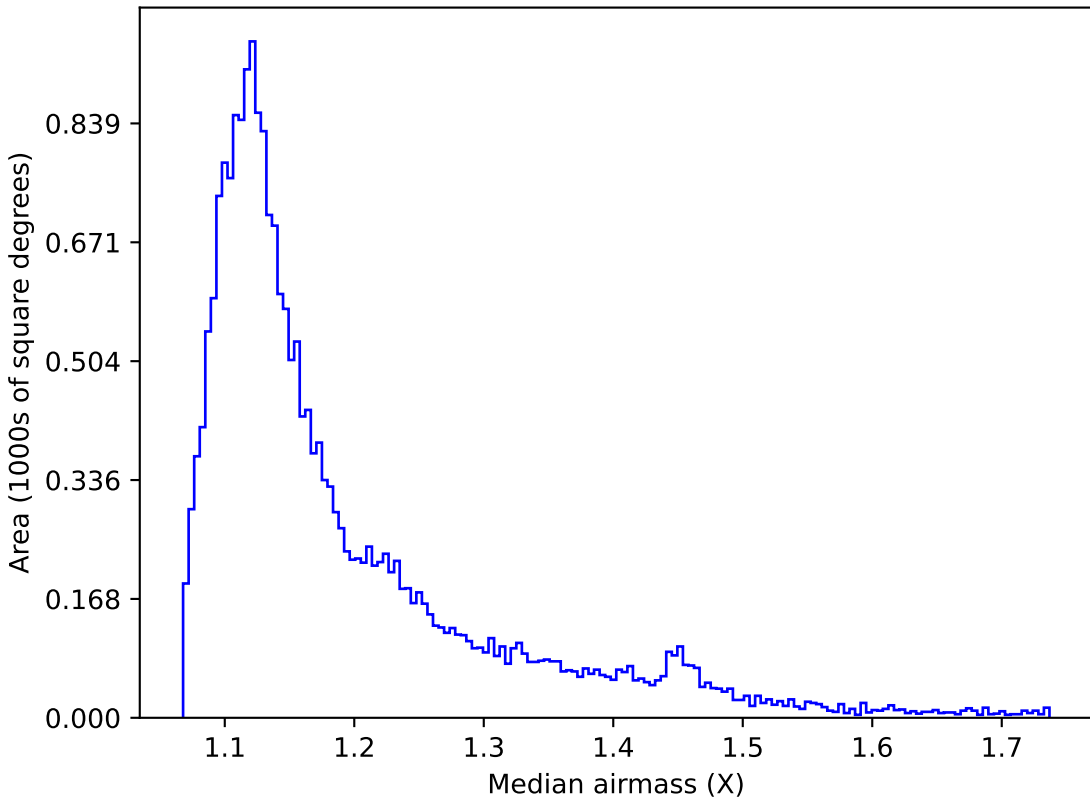
mw_roll_all_v3.3_10yrs All sky u band: Median airmass
