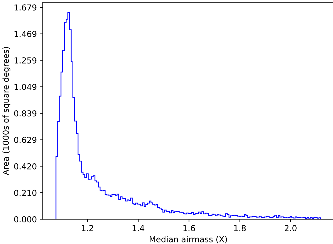
mw_roll_all_v3.3_10yrs All sky r band: Median airmass
