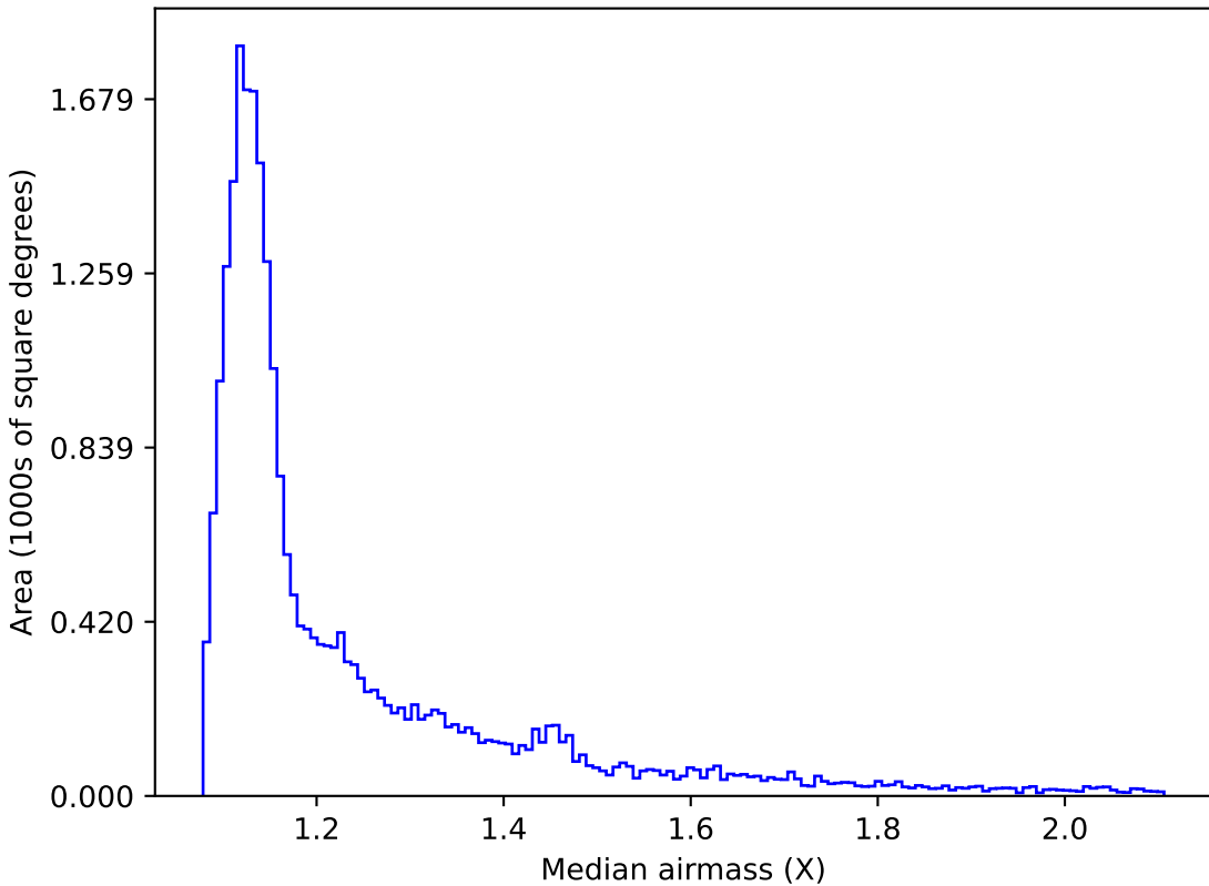
mw_roll_all_v3.3_10yrs All sky i band: Median airmass
