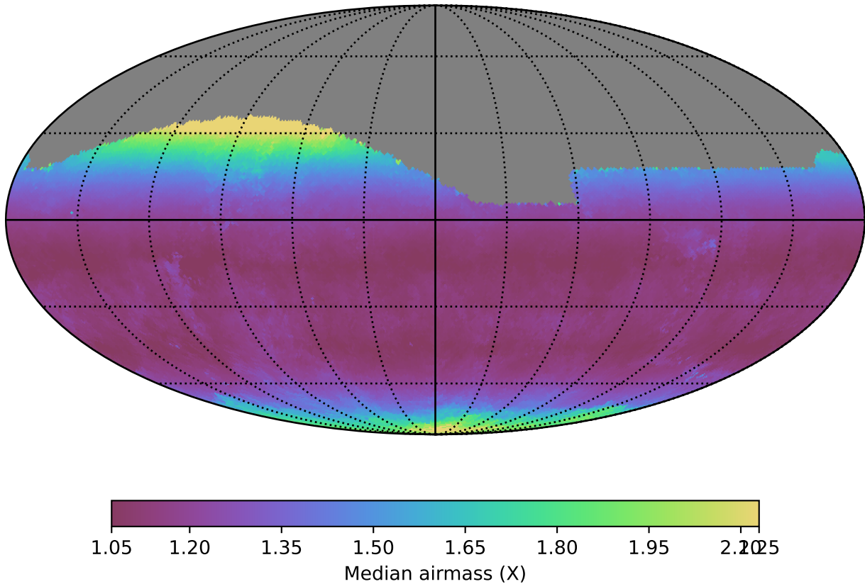
mw_roll_all_v3.3_10yrs All sky g band: Median airmass
