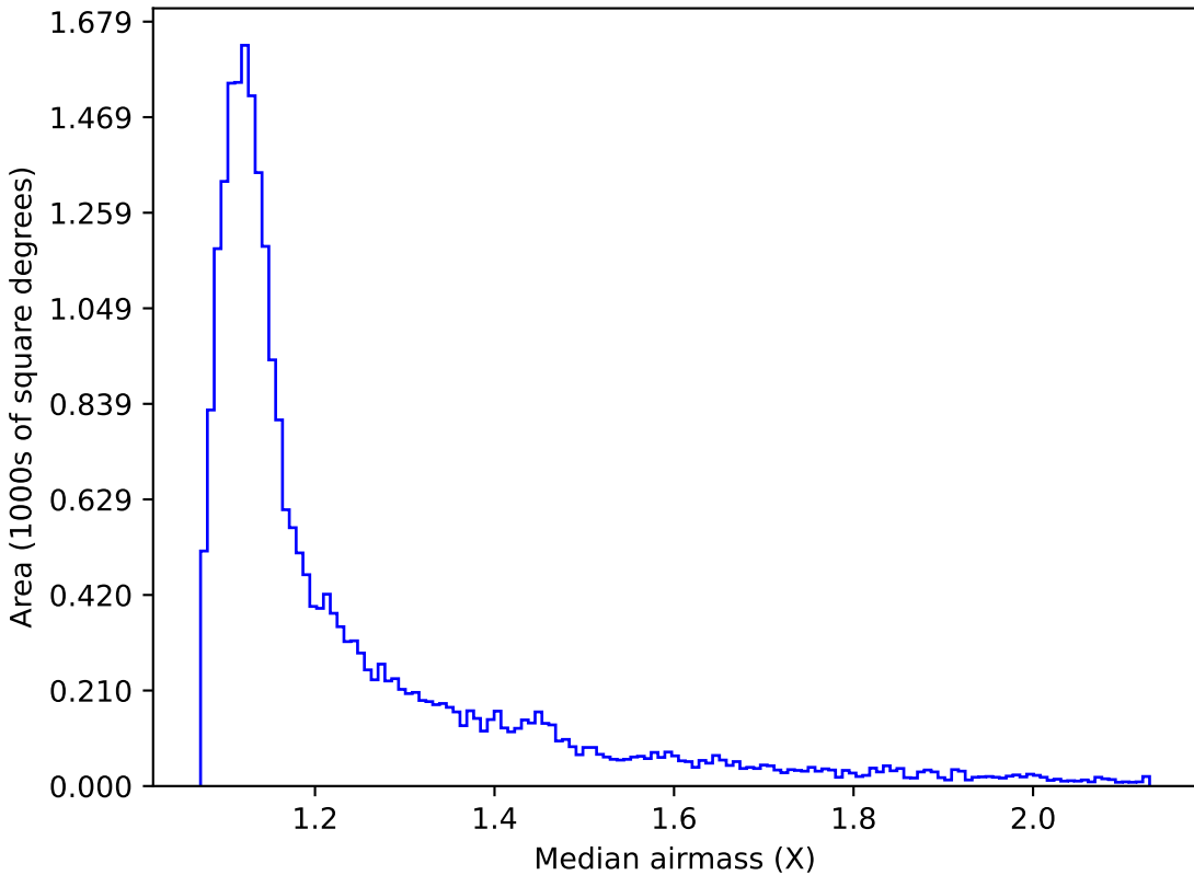
mw_roll_all_v3.3_10yrs All sky g band: Median airmass
