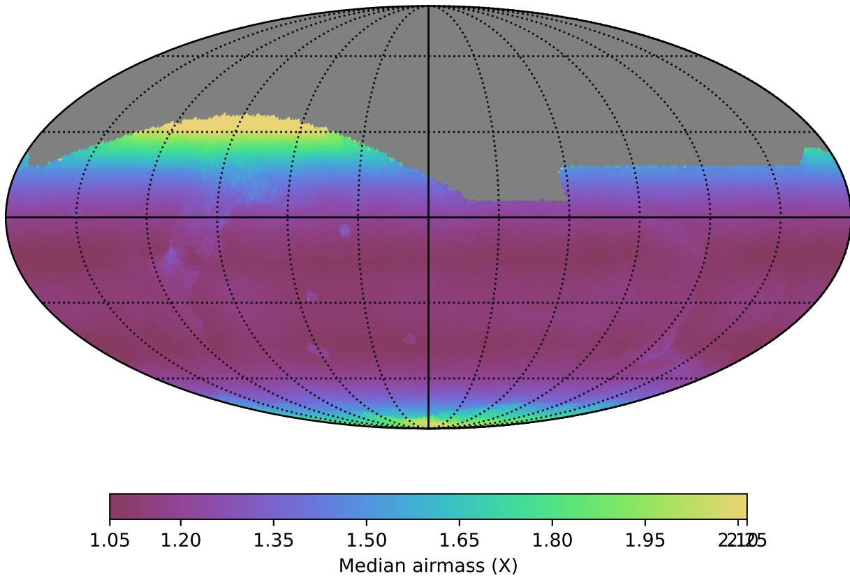
mw_roll_all_v3.3_10yrs All sky all bands: Median airmass
