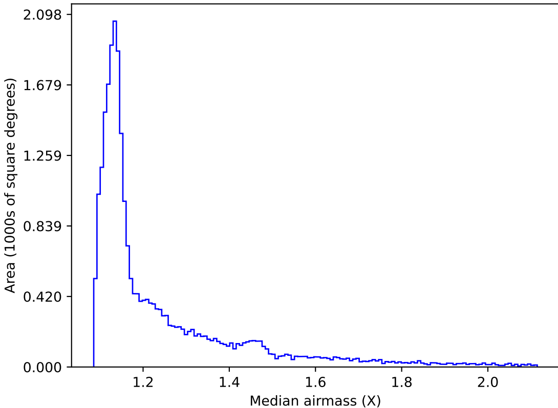
mw_roll_all_v3.3_10yrs All sky all bands: Median airmass
