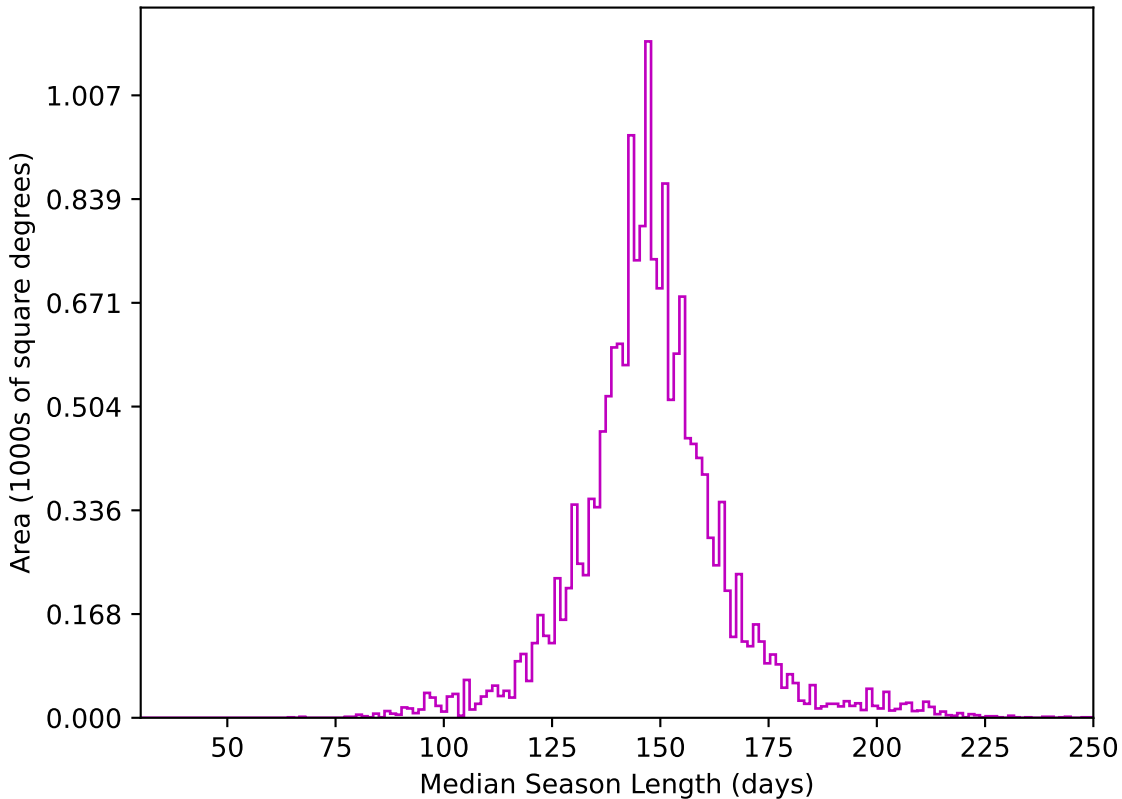
mw_roll_all_v3.3_10yrs WFD z band: Median Season Length
