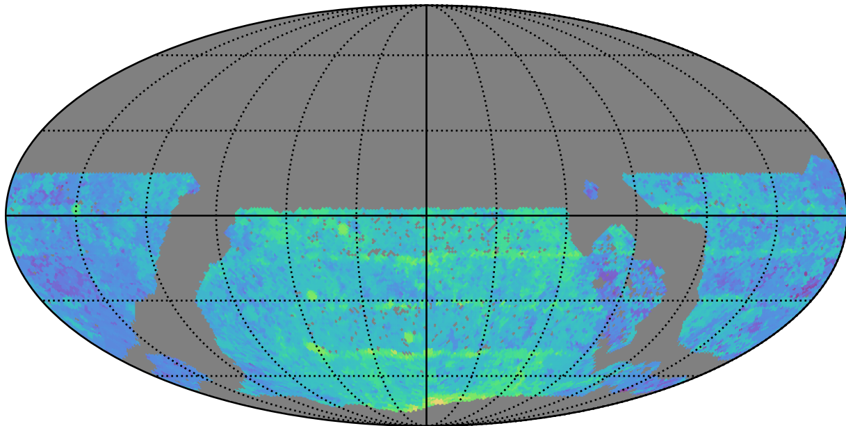
mw_roll_all_v3.3_10yrs WFD y band: Median Season Length
