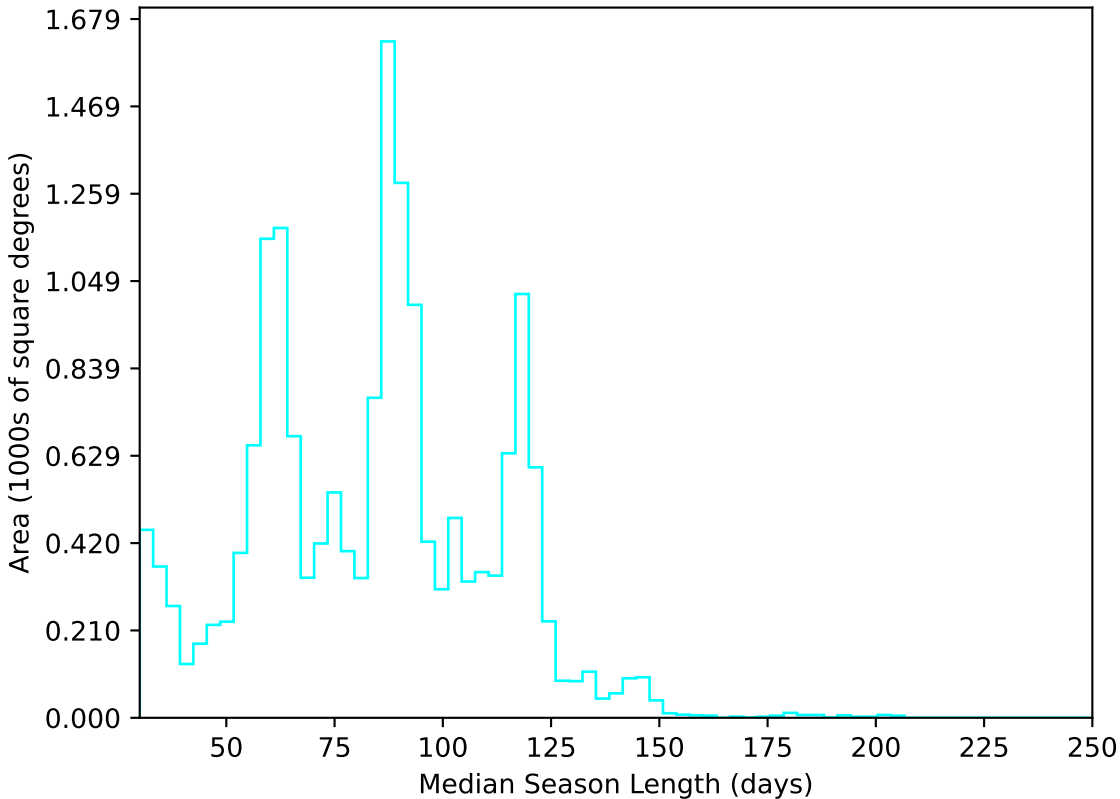
mw_roll_all_v3.3_10yrs WFD u band: Median Season Length
