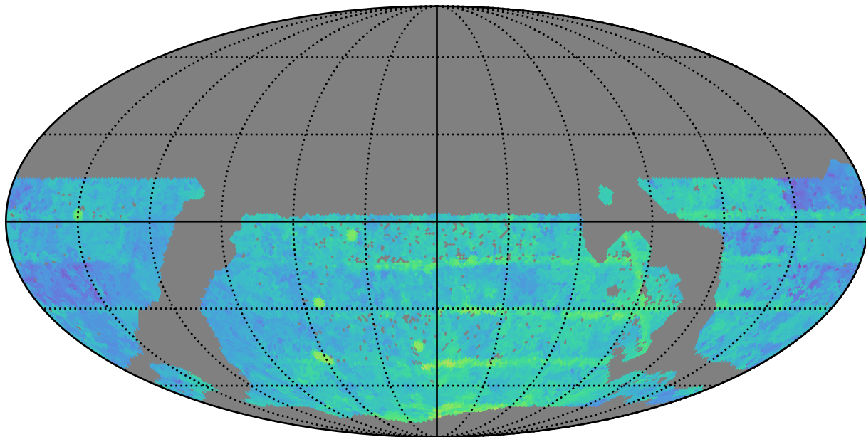
mw_roll_all_v3.3_10yrs WFD r band: Median Season Length
