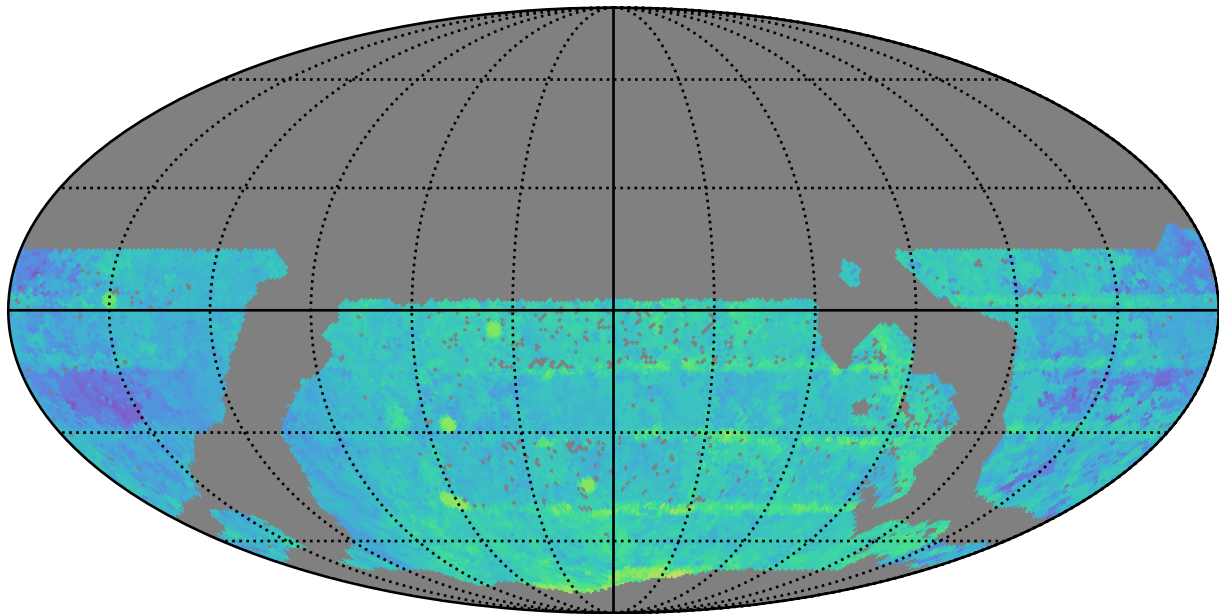
mw_roll_all_v3.3_10yrs WFD i band: Median Season Length
