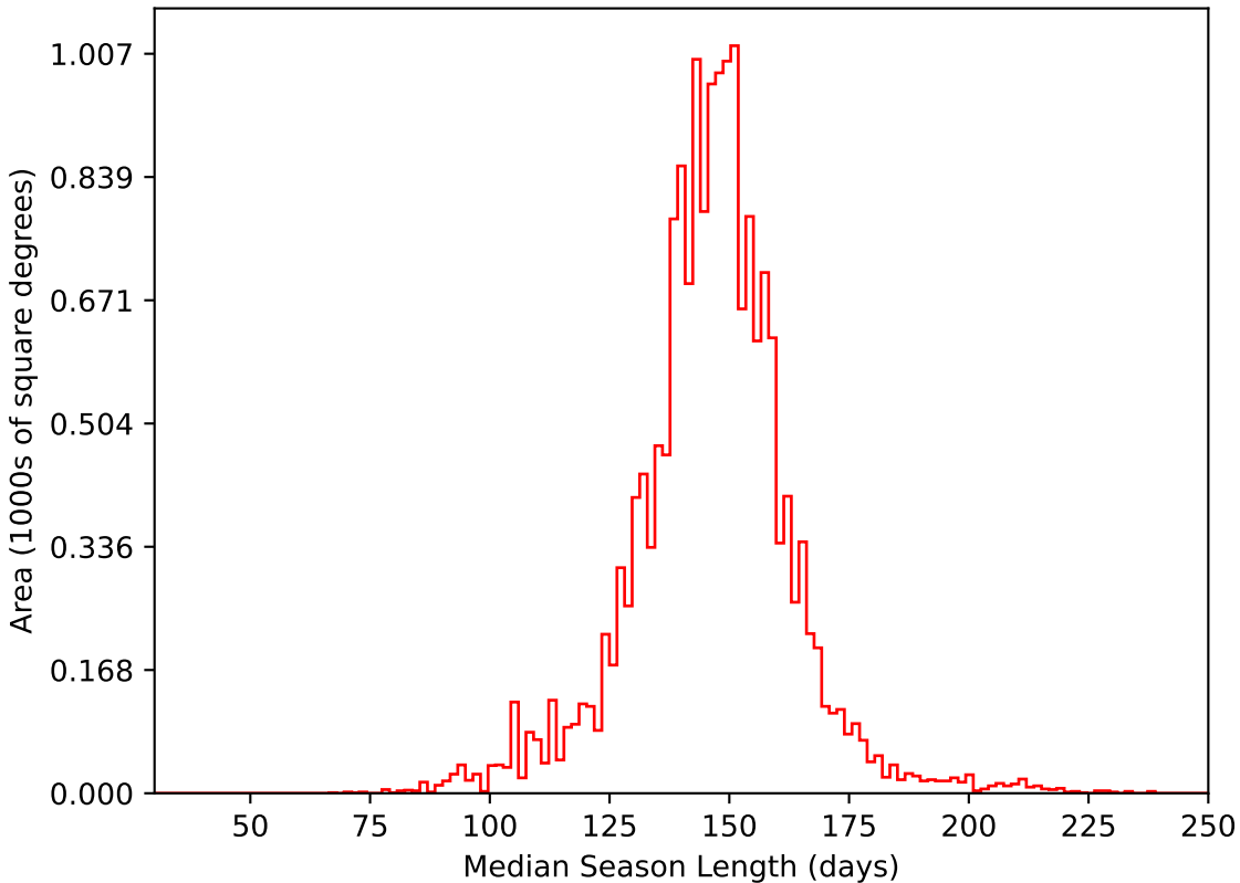
mw_roll_all_v3.3_10yrs WFD i band: Median Season Length
