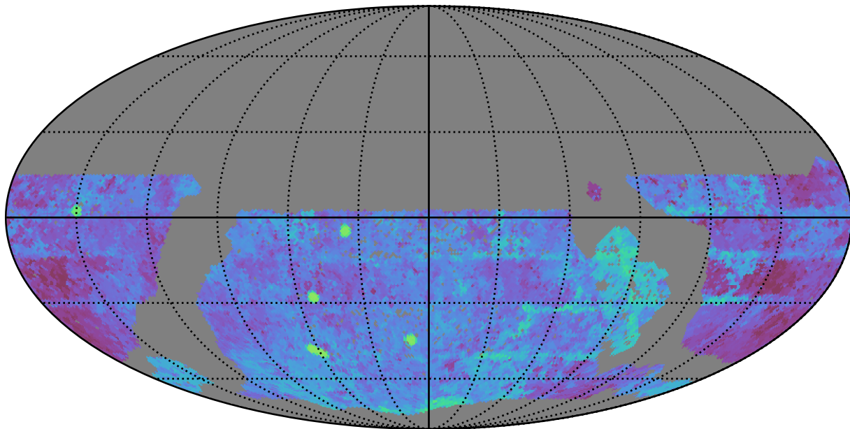
mw_roll_all_v3.3_10yrs WFD g band: Median Season Length
