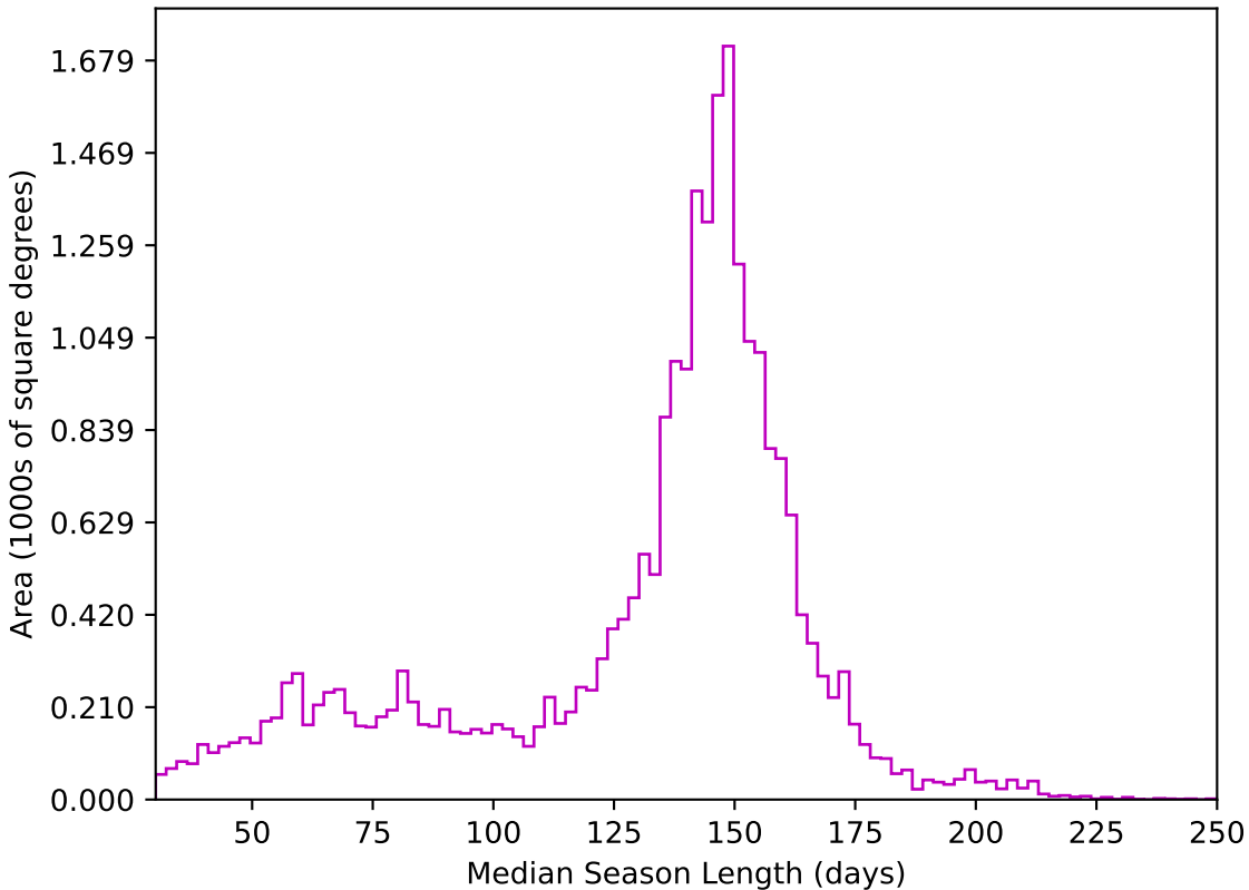
mw_roll_all_v3.3_10yrs All sky z band: Median Season Length
