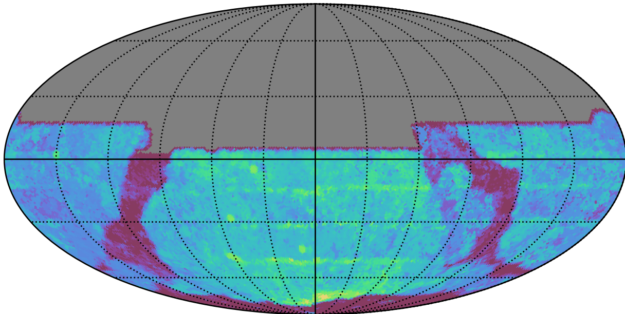
mw_roll_all_v3.3_10yrs All sky y band: Median Season Length
