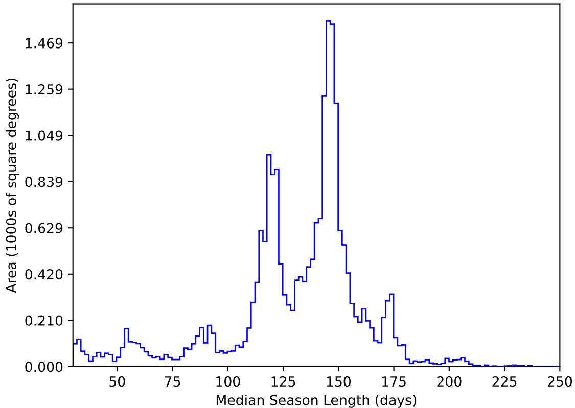
mw_roll_all_v3.3_10yrs All sky y band: Median Season Length
