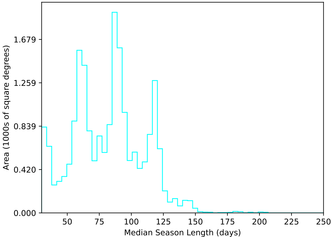
mw_roll_all_v3.3_10yrs All sky u band: Median Season Length
