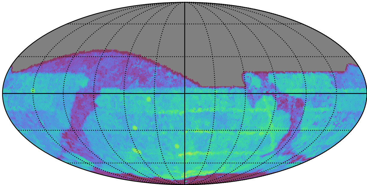
mw_roll_all_v3.3_10yrs All sky r band: Median Season Length
