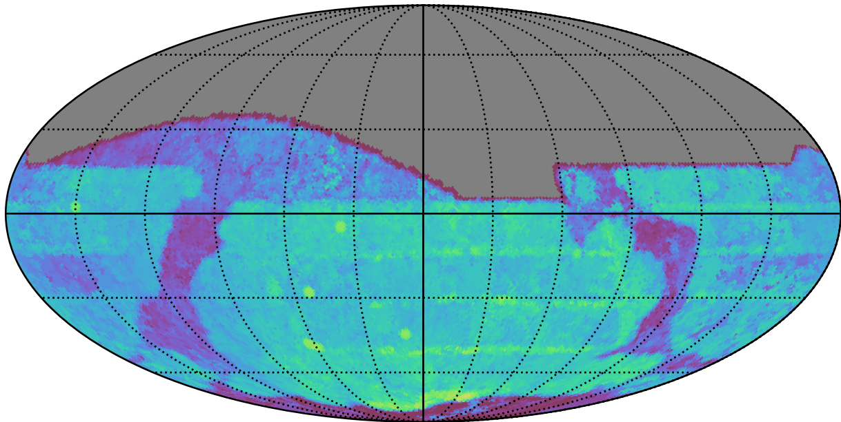
mw_roll_all_v3.3_10yrs All sky i band: Median Season Length
