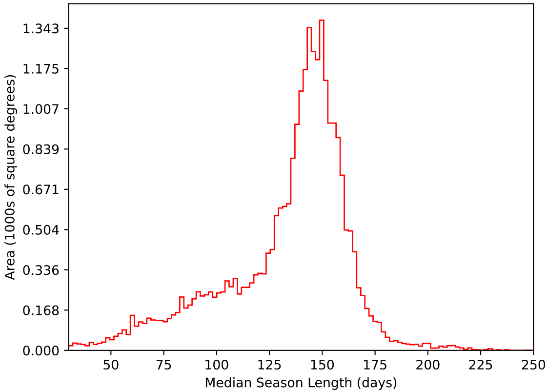
mw_roll_all_v3.3_10yrs All sky i band: Median Season Length
