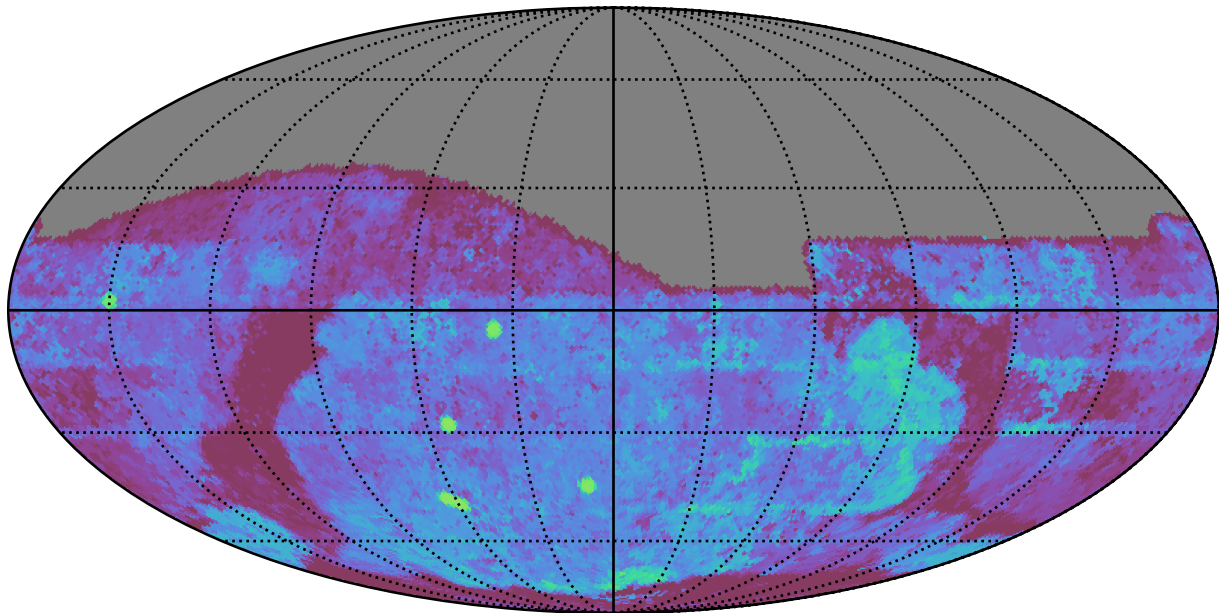
mw_roll_all_v3.3_10yrs All sky g band: Median Season Length
