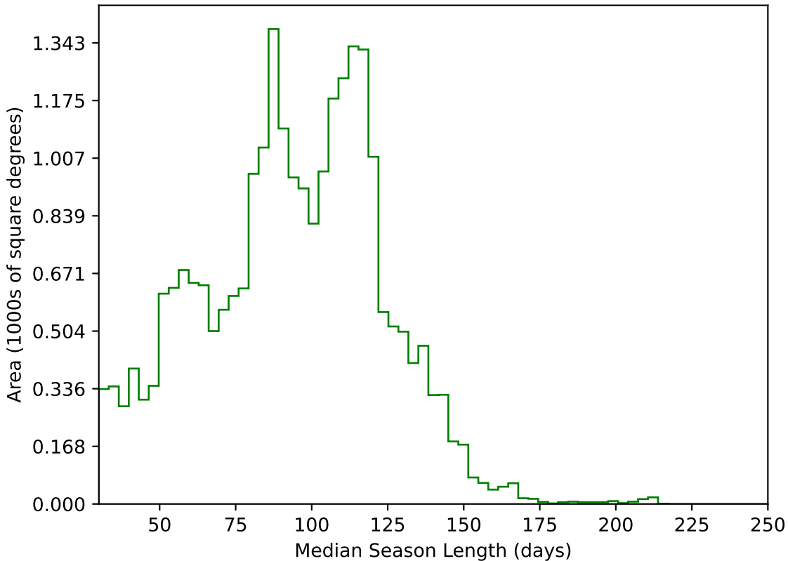
mw_roll_all_v3.3_10yrs All sky g band: Median Season Length
