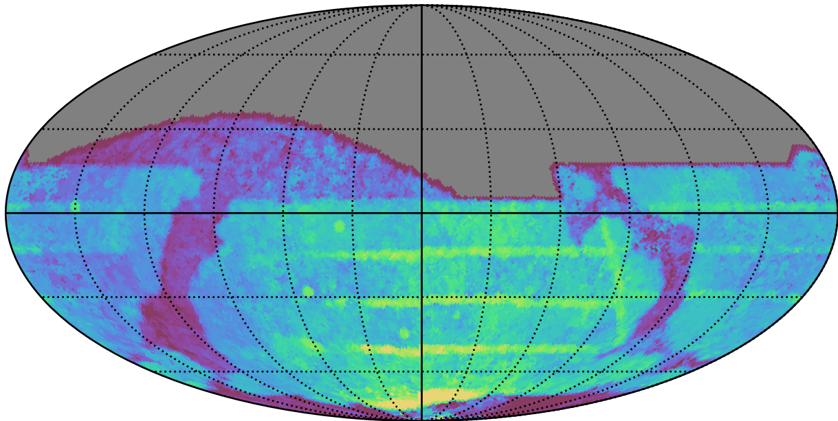
mw_roll_all_v3.3_10yrs All sky all bands: Median Season Length
