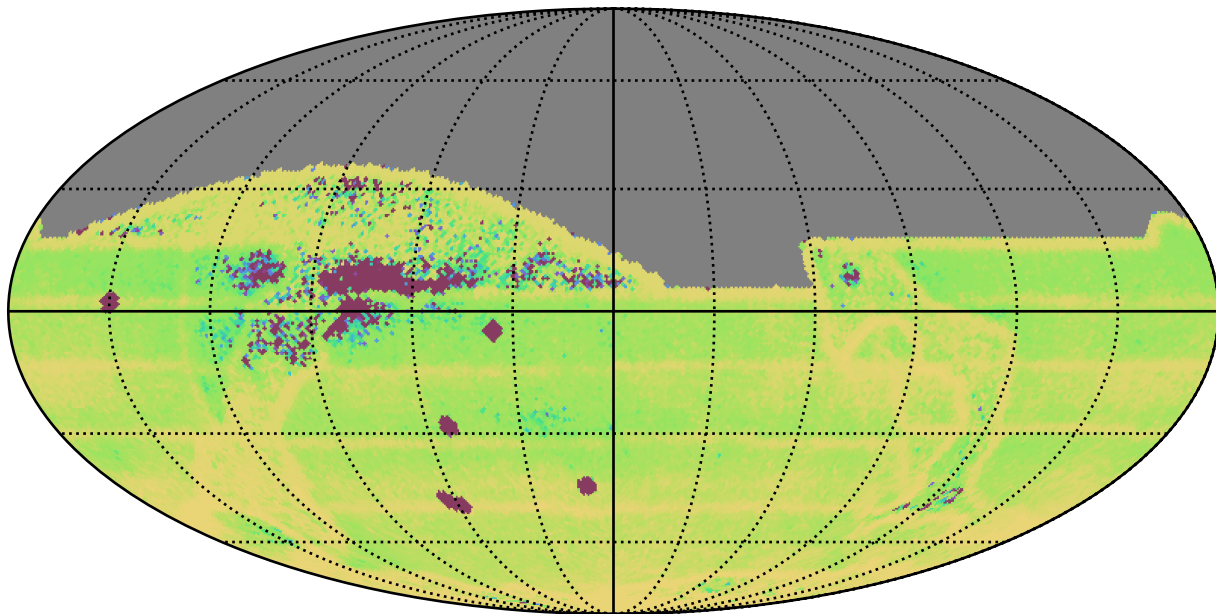
mw_roll_all_v3.3_10yrs All sky: Median Intra-Night Gap
