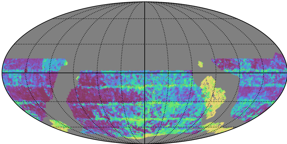
mw_roll_all_v3.3_10yrs WFD y band: Median Inter-Night Gap
