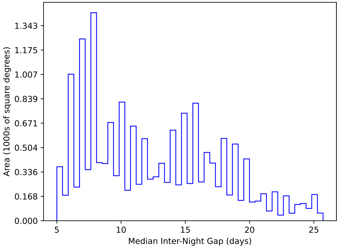
mw_roll_all_v3.3_10yrs WFD y band: Median Inter-Night Gap
