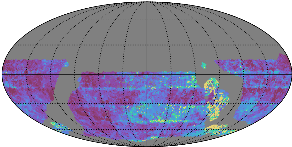
mw_roll_all_v3.3_10yrs WFD u band: Median Inter-Night Gap
