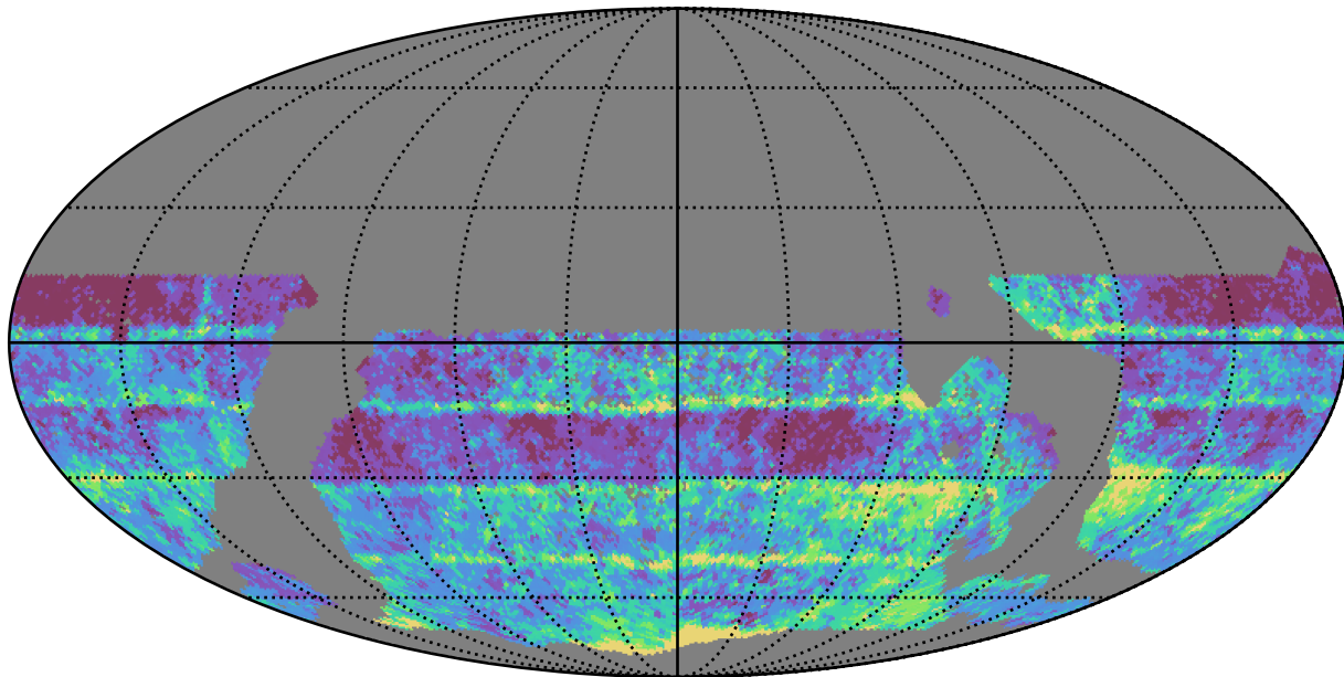
mw_roll_all_v3.3_10yrs WFD r band: Median Inter-Night Gap
