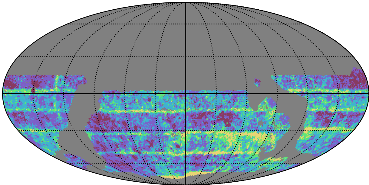
mw_roll_all_v3.3_10yrs WFD i band: Median Inter-Night Gap
