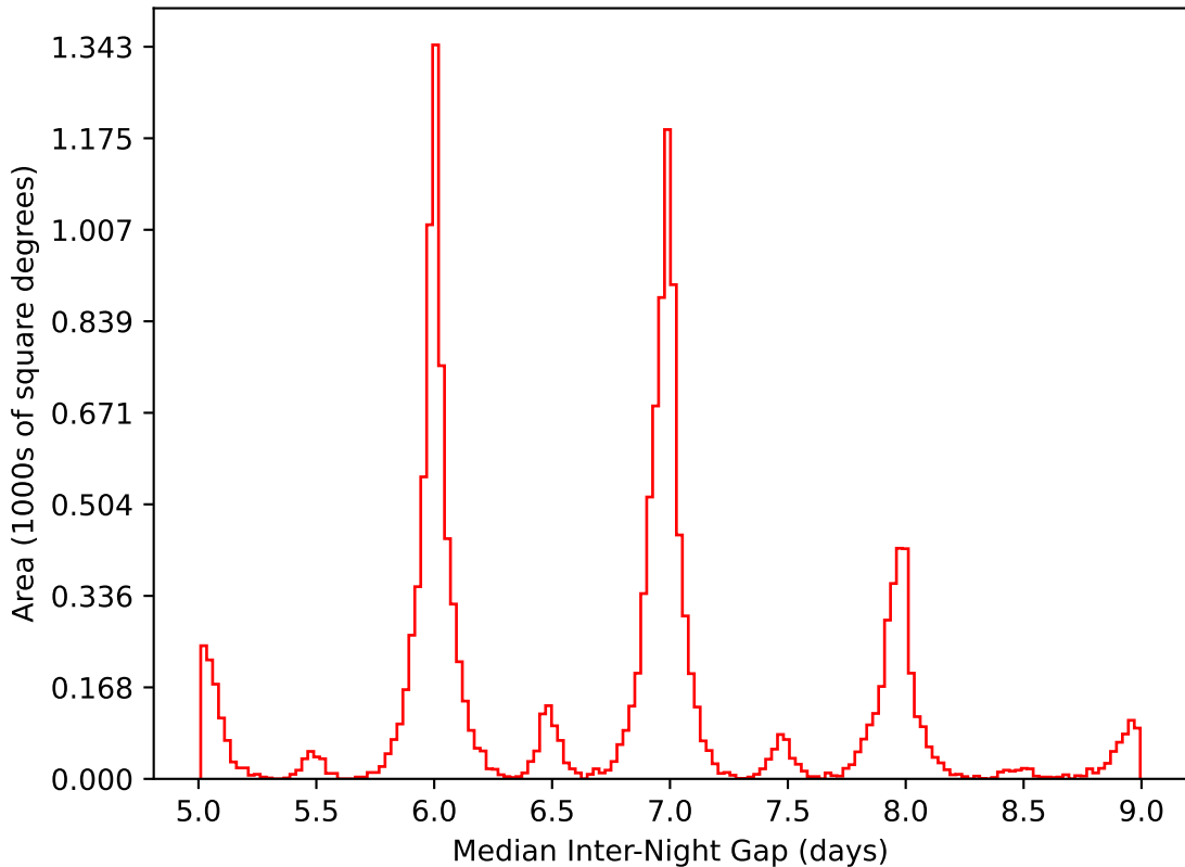
mw_roll_all_v3.3_10yrs WFD i band: Median Inter-Night Gap
