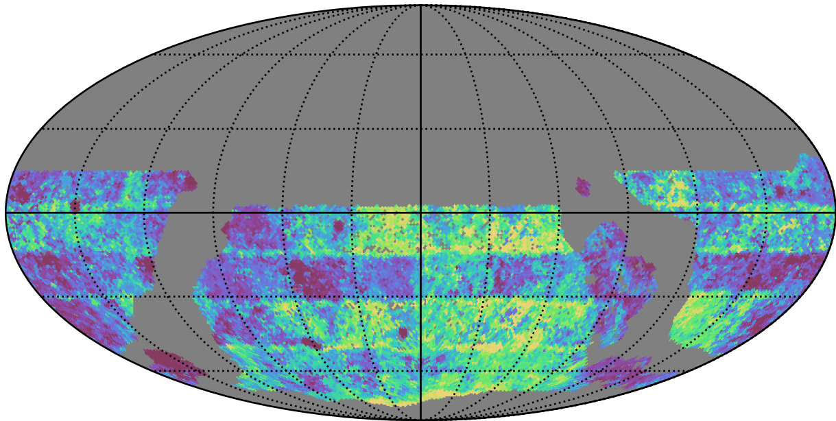
mw_roll_all_v3.3_10yrs WFD g band: Median Inter-Night Gap
