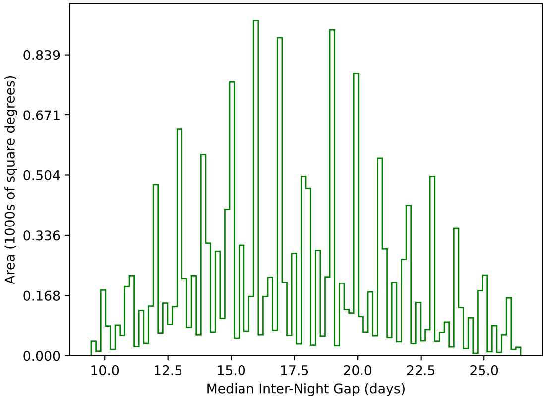
mw_roll_all_v3.3_10yrs WFD g band: Median Inter-Night Gap
