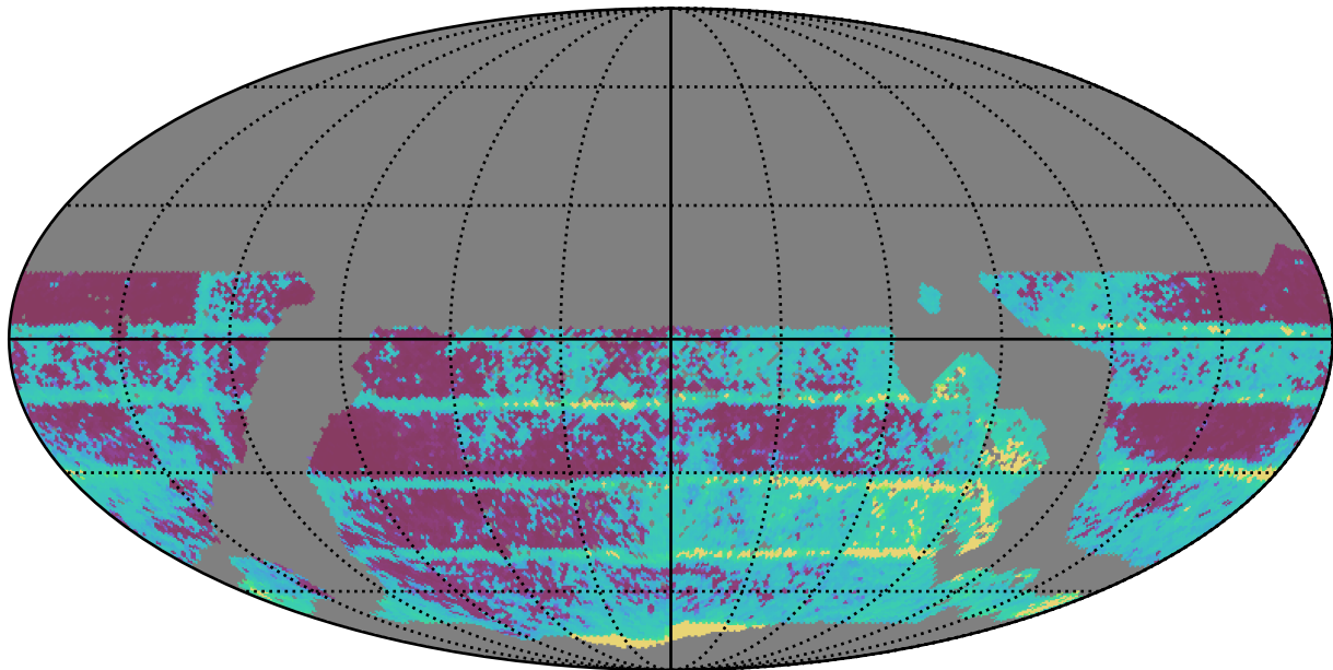
mw_roll_all_v3.3_10yrs WFD all bands: Median Inter-Night Gap
