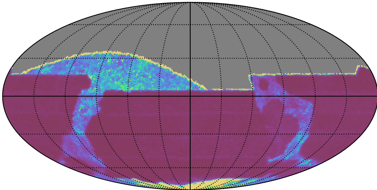
mw_roll_all_v3.3_10yrs All sky z band: Median Inter-Night Gap
