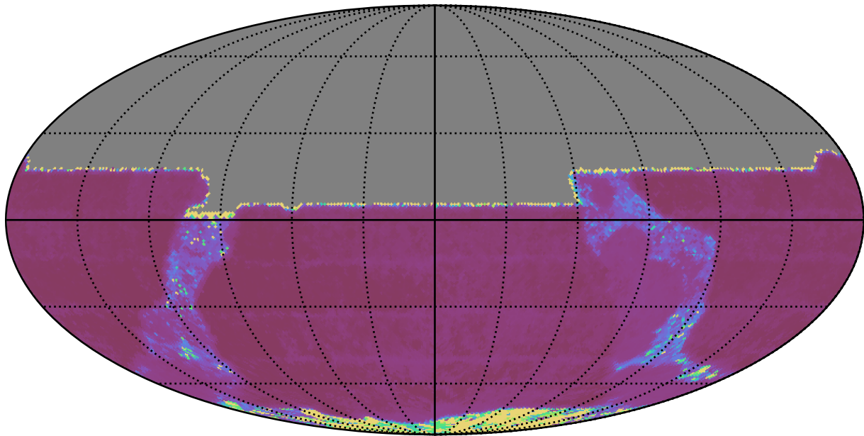
mw_roll_all_v3.3_10yrs All sky y band: Median Inter-Night Gap
