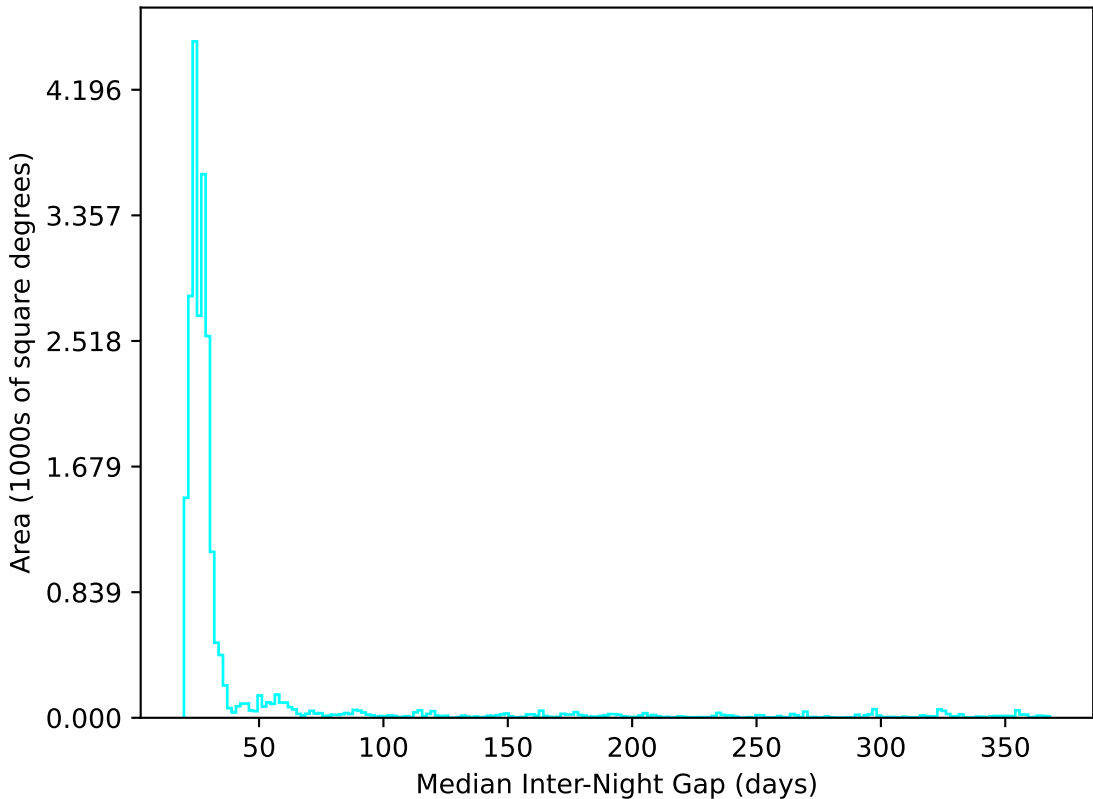
mw_roll_all_v3.3_10yrs All sky u band: Median Inter-Night Gap
