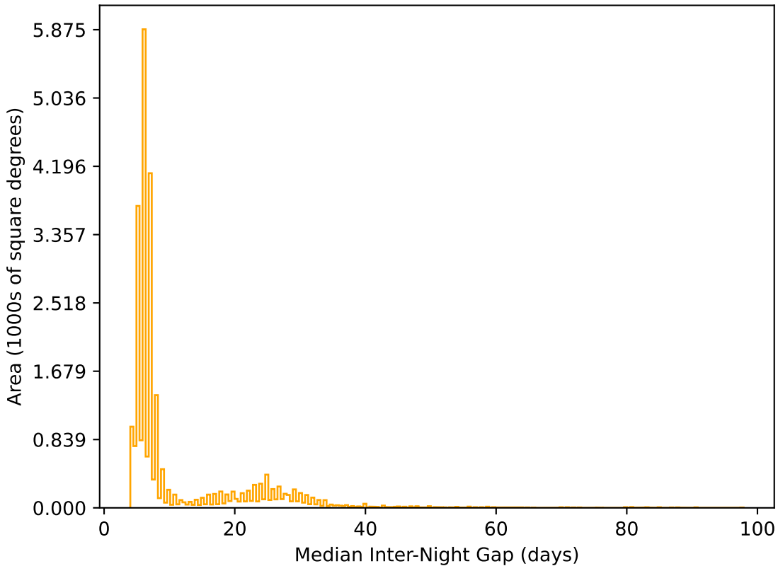
mw_roll_all_v3.3_10yrs All sky r band: Median Inter-Night Gap
