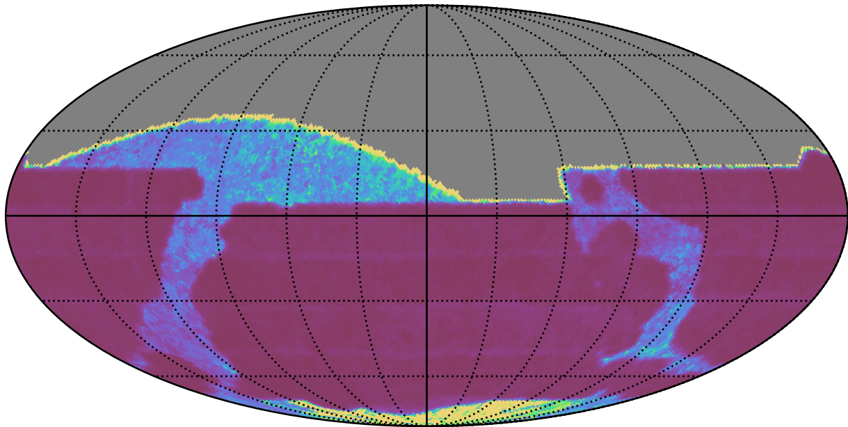
mw_roll_all_v3.3_10yrs All sky i band: Median Inter-Night Gap
