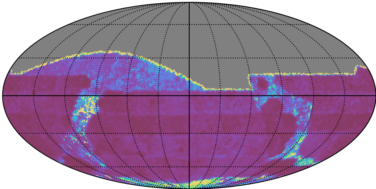
mw_roll_all_v3.3_10yrs All sky g band: Median Inter-Night Gap
