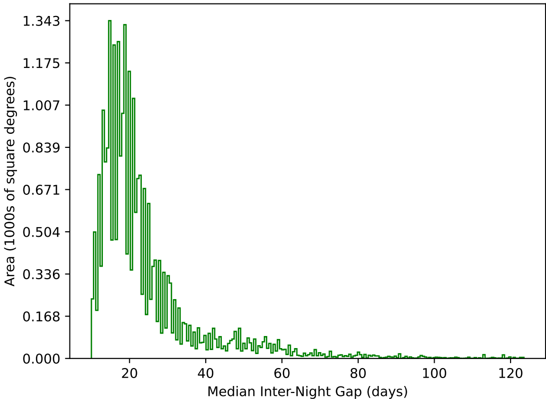
mw_roll_all_v3.3_10yrs All sky g band: Median Inter-Night Gap
