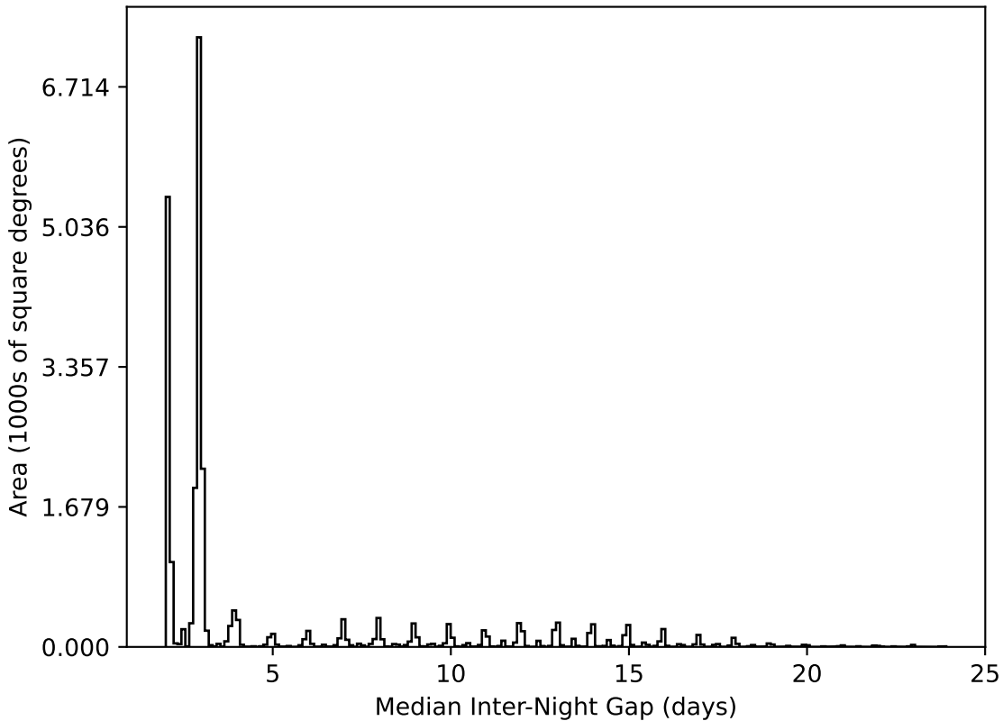
mw_roll_all_v3.3_10yrs All sky all bands: Median Inter-Night Gap
