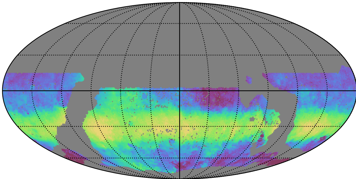
mw_roll_all_v3.3_10yrs WFD z band: Median HA
