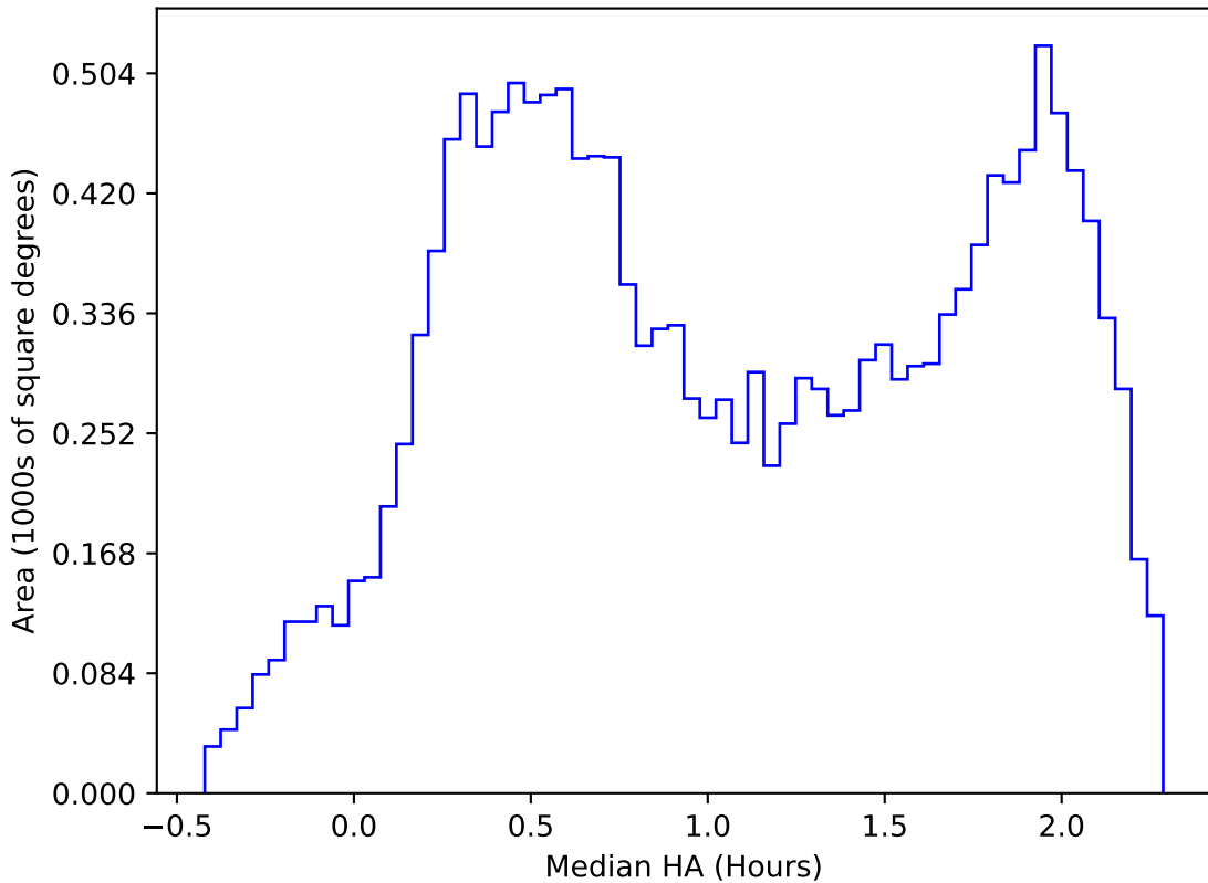
mw_roll_all_v3.3_10yrs WFD z band: Median HA
