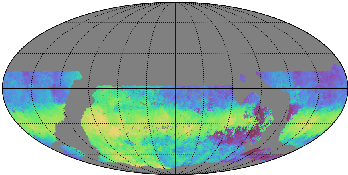
mw_roll_all_v3.3_10yrs WFD u band: Median HA
