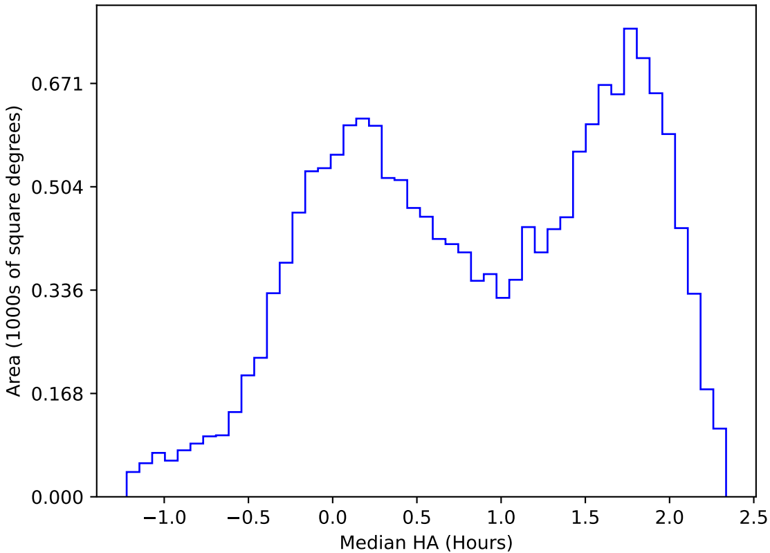
mw_roll_all_v3.3_10yrs WFD u band: Median HA
